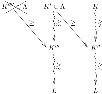
(e) The only possible scenario when K \gtrsim L holds but K does not produce L in \Lambda : some literal K' \in \Lambda shields L from K , and K' strongly covers \bar{L} in \Lambda (and hence produces \bar{L} in \Lambda ).
