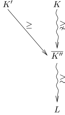
(b) K' shields L from K .
